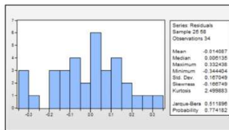
Gambar.6. Output Uji Asumsi Normalitas Residual Model SARIMA(2,1,2)(2,1,1) 7
