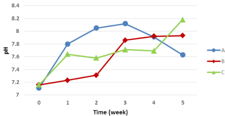
Figure 1. Changes in substrate pH during anaerobic breakdown at thermophilic temperature
