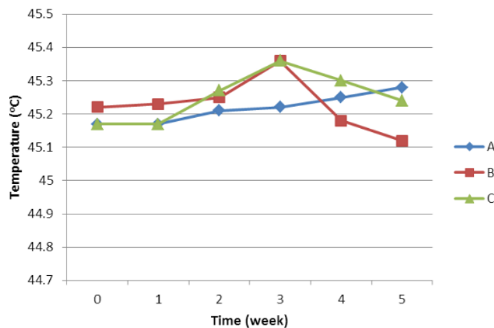
Figure 2. Changes in substrate temperature during the thermophilic temperature anaerobic reform process
