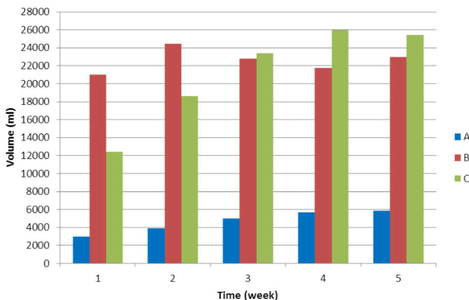
Figure 3. Volume of biogas resulting from anaerobic remodeling at thermophilic temperature
