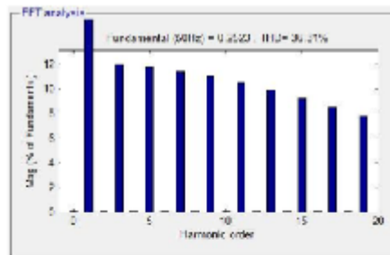
Figure 6. Current harmonic spectrum simulation results
