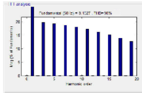
Figure 4. Current harmonic spectrum simulation results
