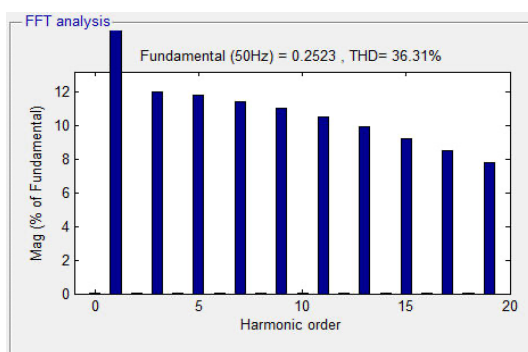
Figure 6. Current harmonic spectrum simulation results
