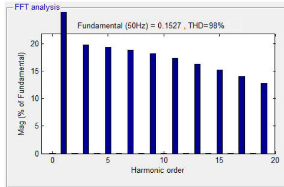
Figure 4. Current harmonic spectrum simulation results
