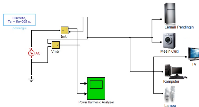
Figure 2. Non-linear loading simulation
